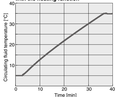
Temperature increase with the heating function
