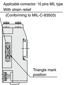
60PH (10 pins)
