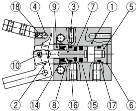
Double acting/With fingers open
