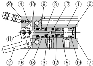
Double acting/With fingers open
