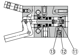
Double acting/With fingers closed Single acting
