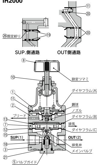
IR2120
