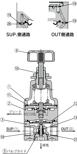
IR1000
